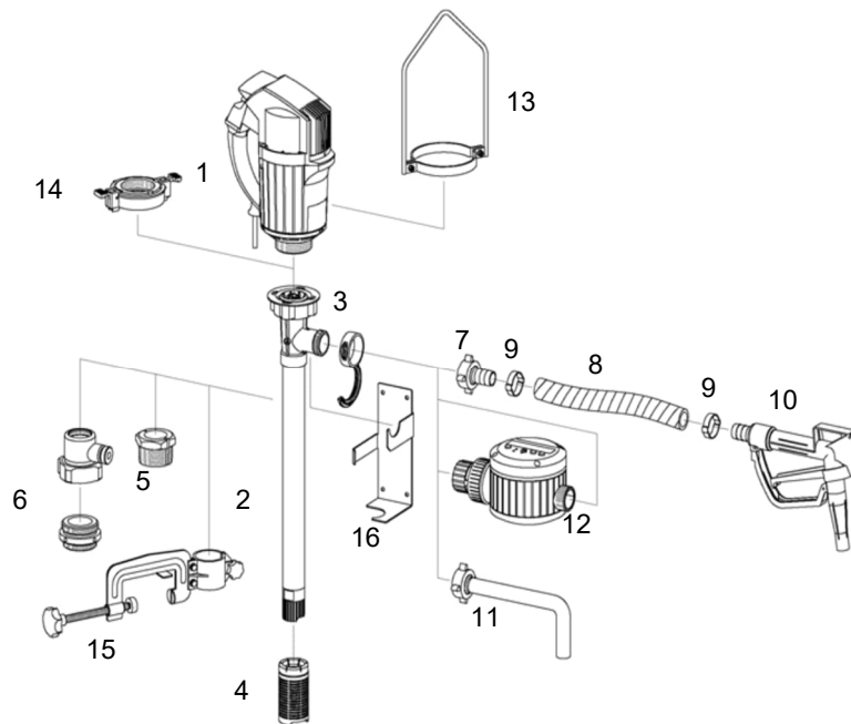
Fig. 1 Layout of pump (with components), non-explosion-proof
